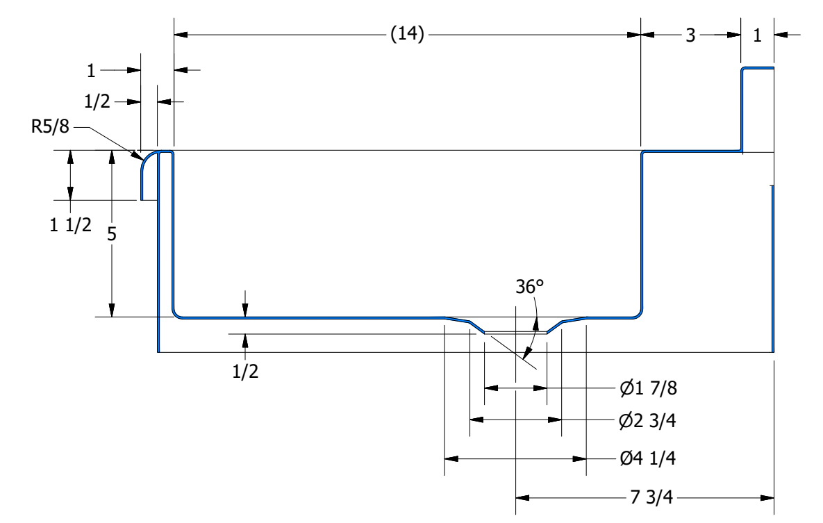
SECTION A-A SCALE 1 / 4
